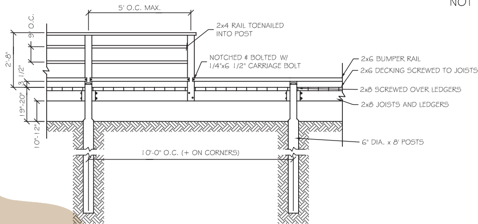
TYPICAL ELEVATION NOT TO SCALE
