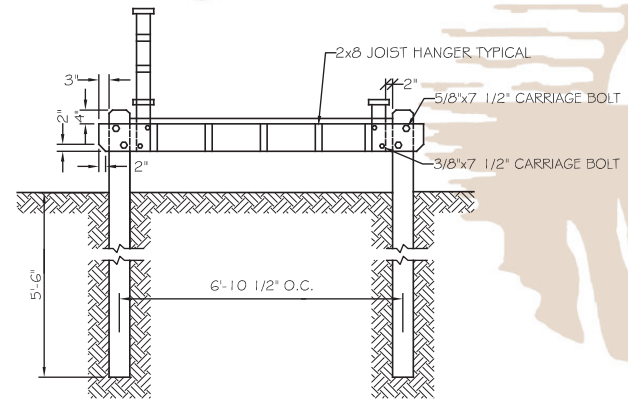
TYPICAL SECTION NOT TO SCALE
