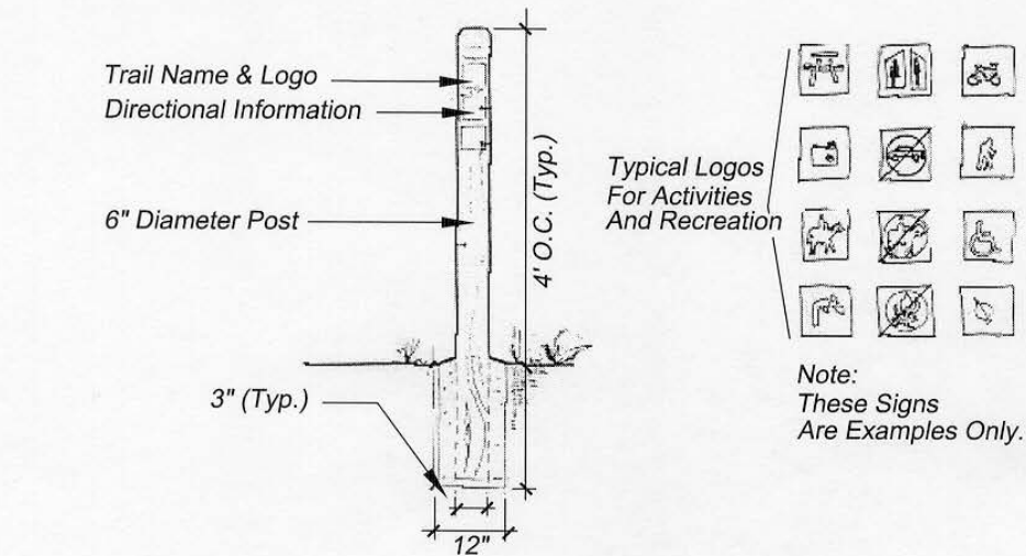
TYPICAL TRAIL MARKER
