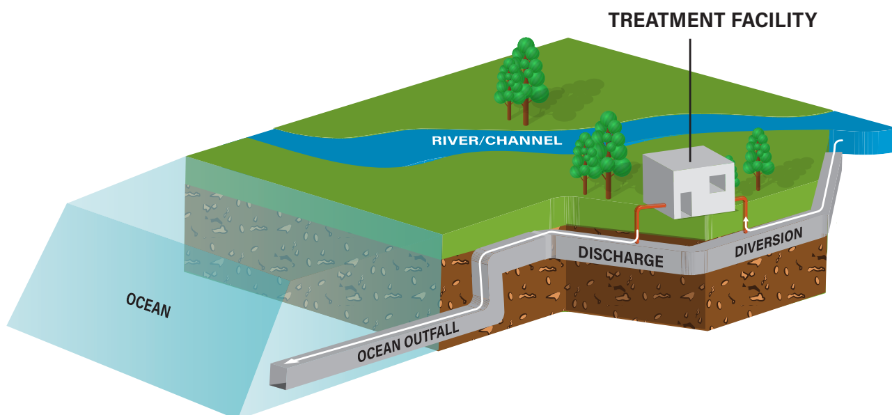
Figure 10: Water Quality Strategy I: Divert and Treat
