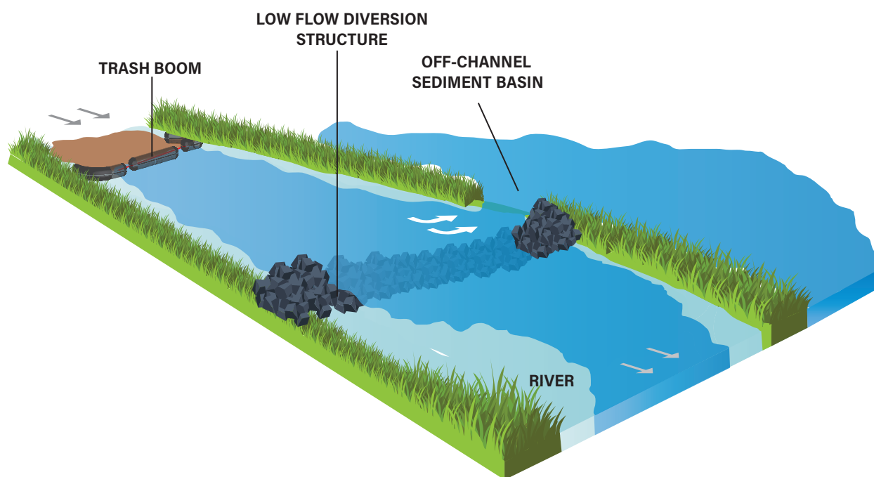
Figure 14: Sediment Capture Strategy II: Off-Channel Basin
