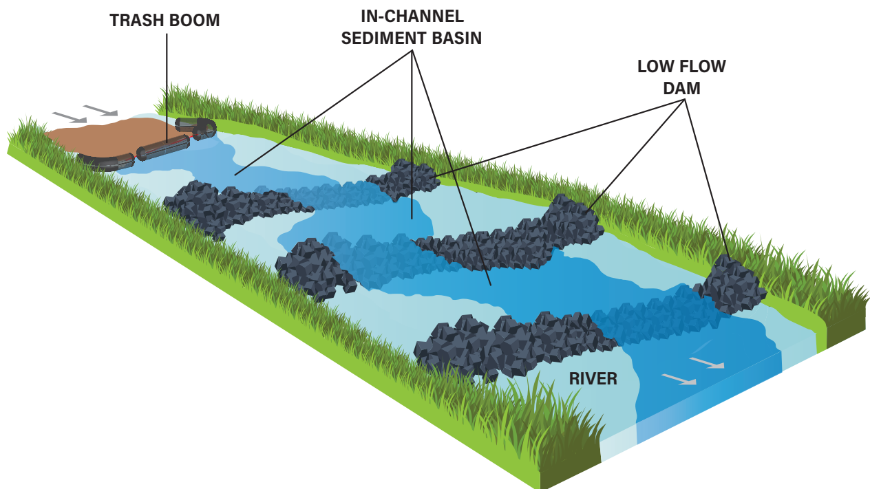
Figure 13: Sediment Capture Strategy I: In-Channel Basin
