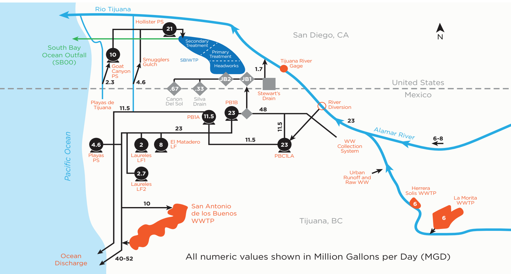
Figure 1: Dry weather Flow Infrastructure on the Tijuana River
