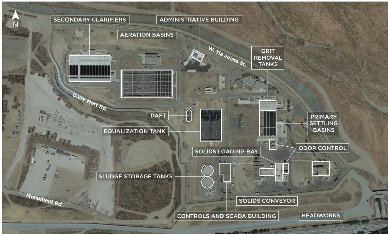
Figure 3: Layout of South Bay International Wastewater Treatment Plant
