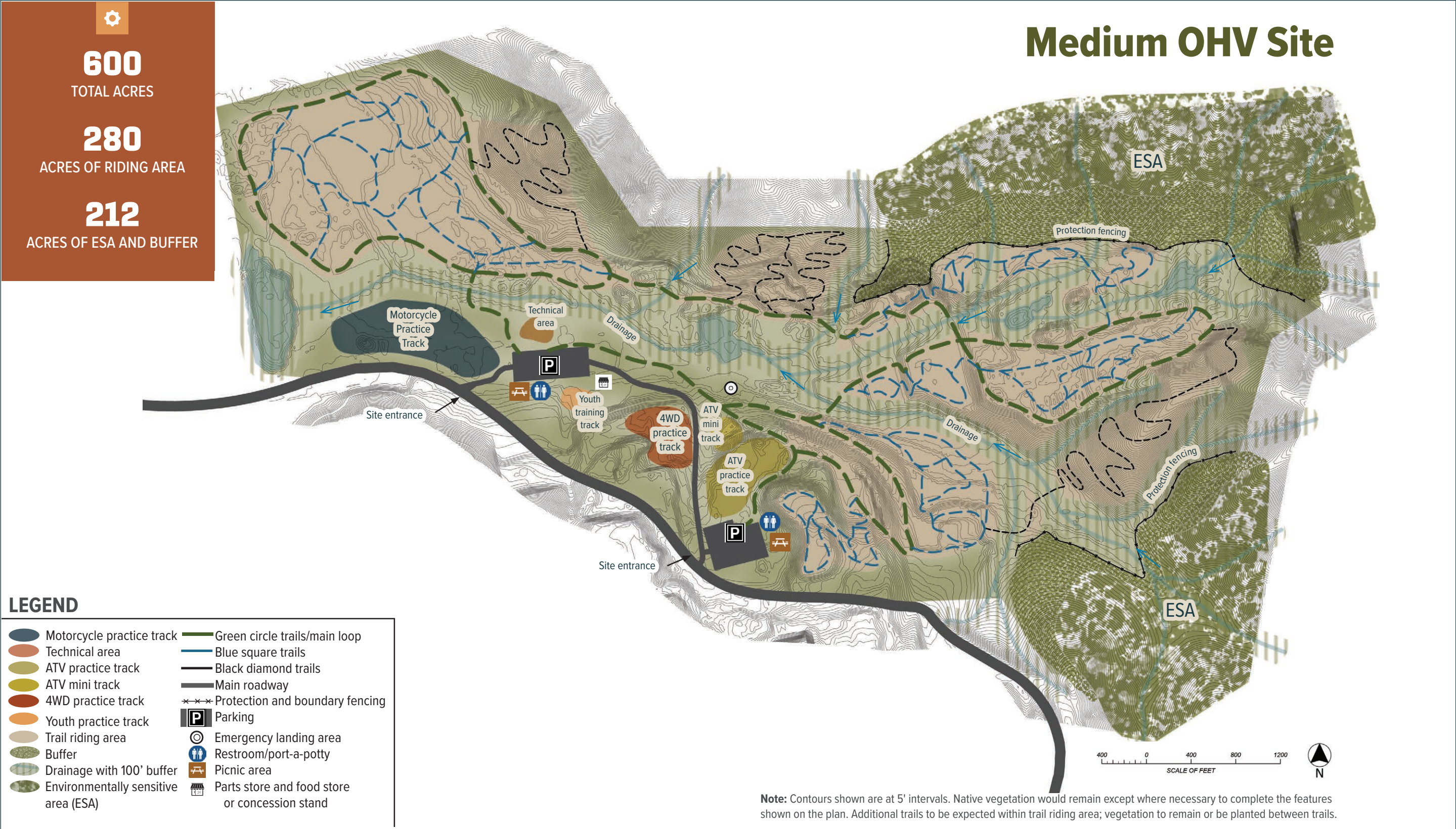
Figure 7-2. Medium OHV Site Conceptual Plan
