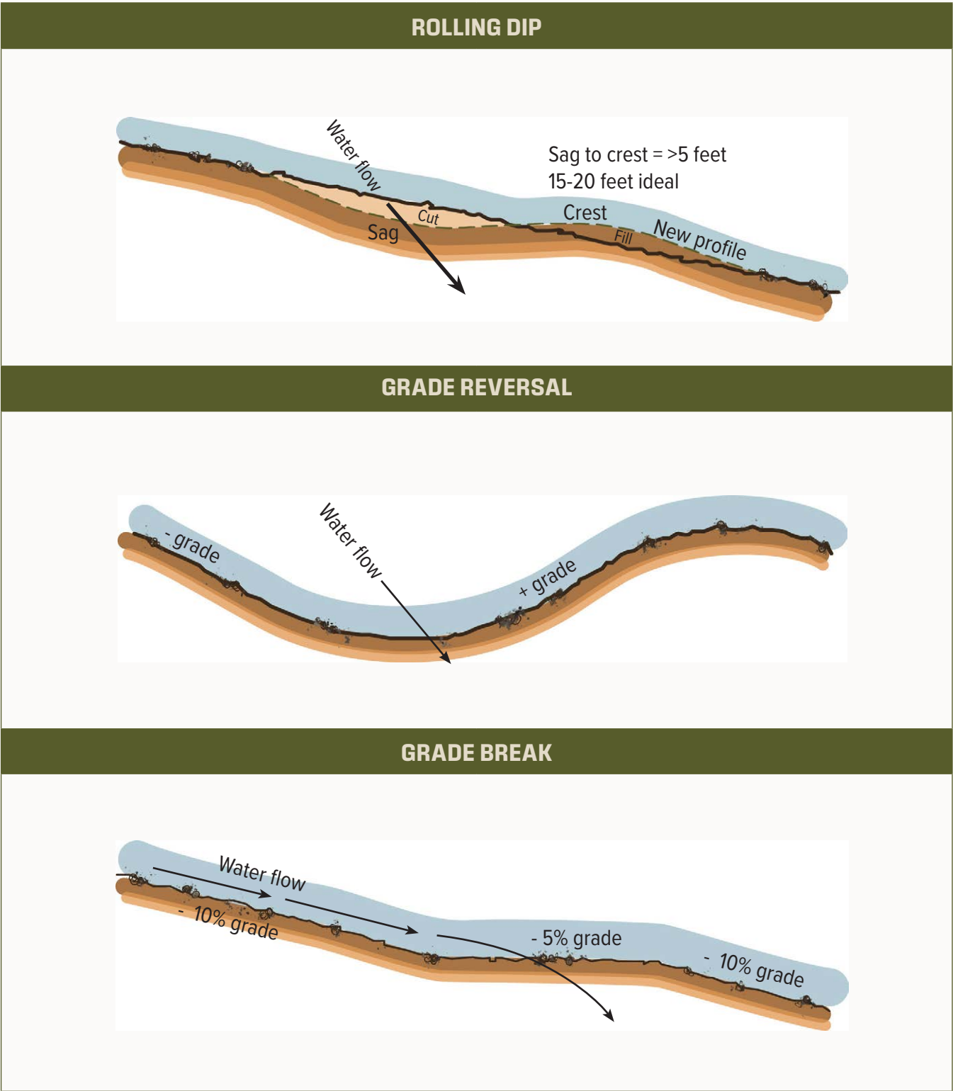
Figure 6-6. Trail Design and Erosion Prevention Measures
